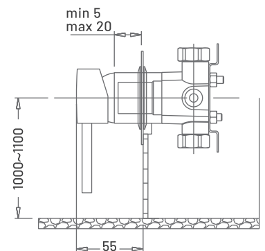
bracket Bath
