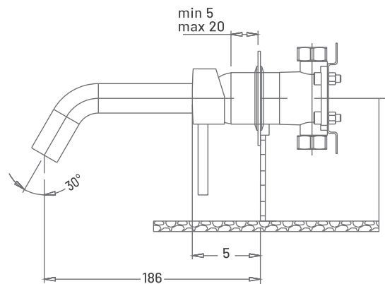
bracket basin
